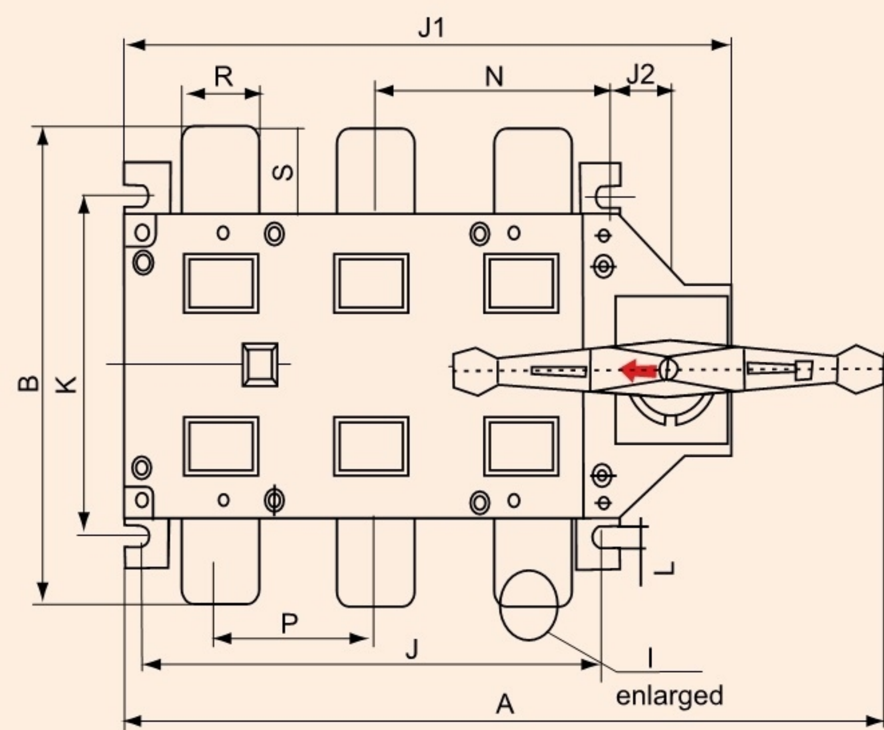
Direct operation of 125~1600A
