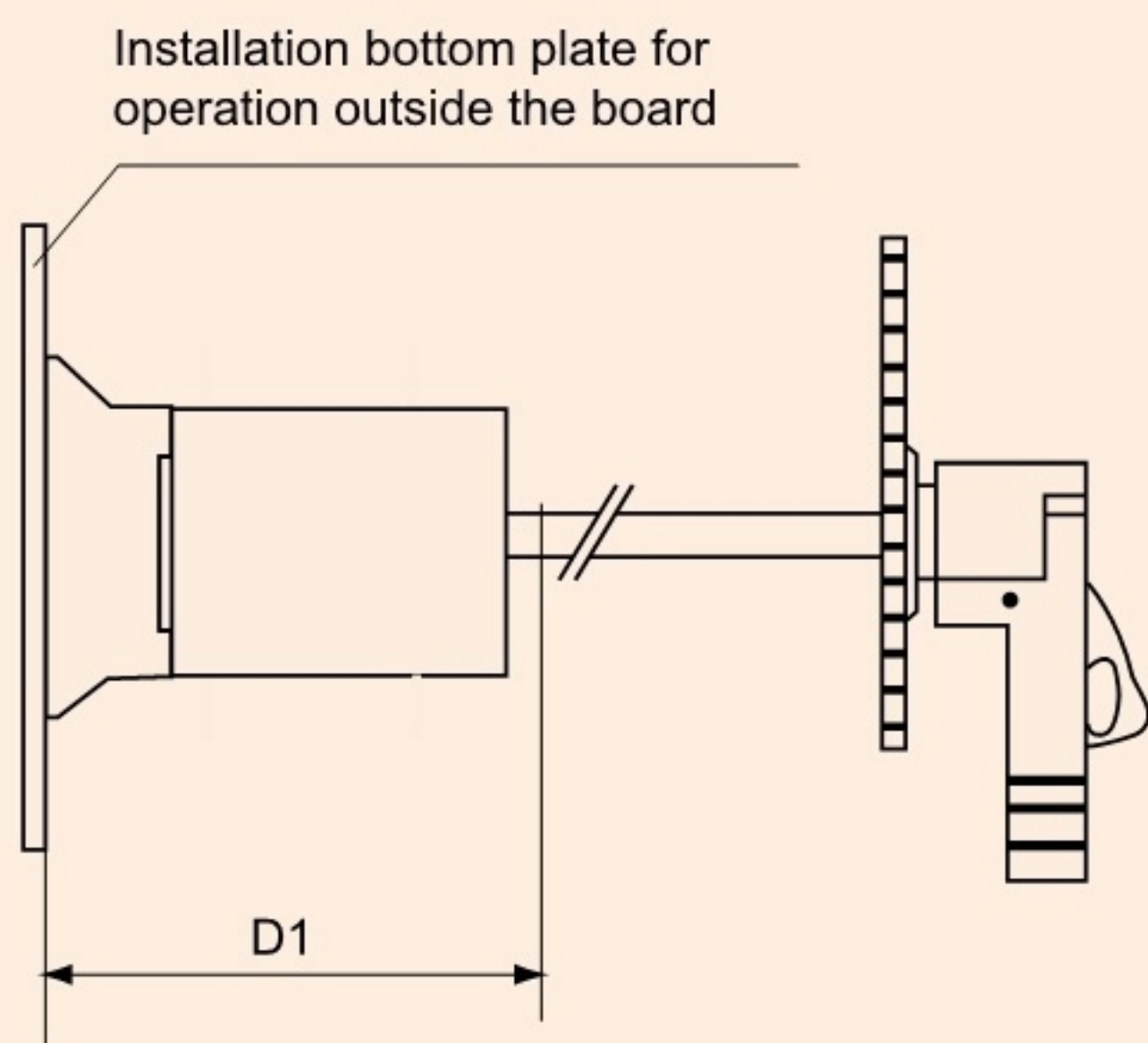
Operation outside 125~1600A/J board
