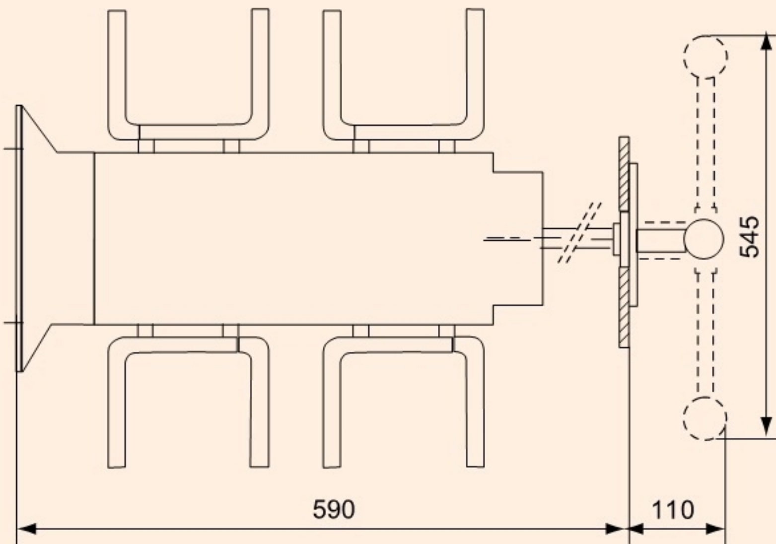
Direct operation on front face 315A/J board
