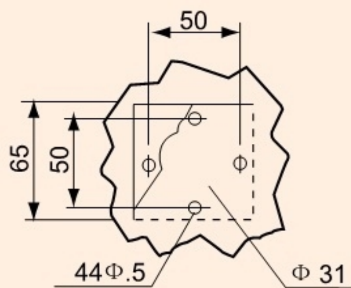
Locking the cabinet face with the lock
