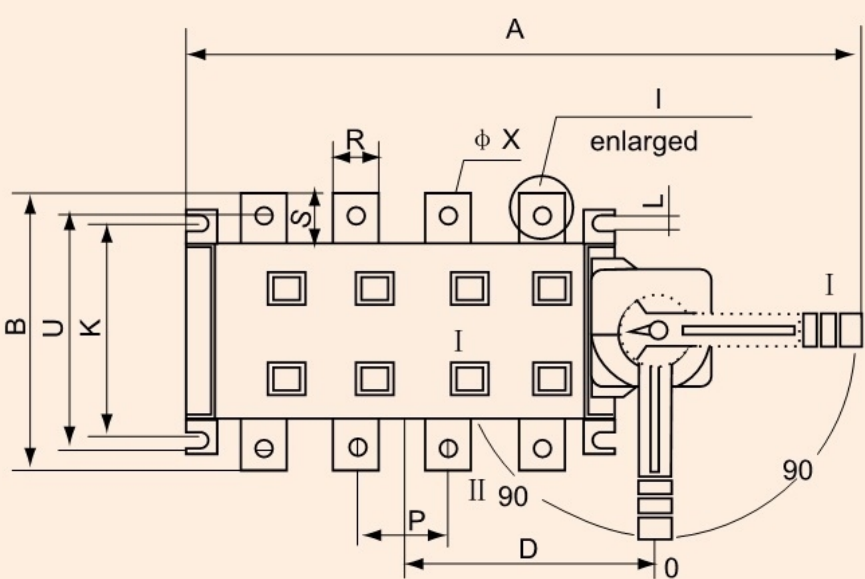
Direct operation of 80~630A
