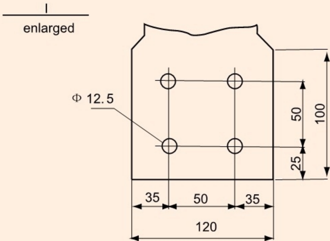
3150~4000A
