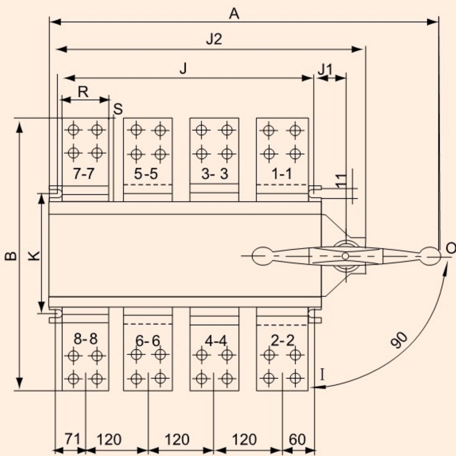
Direct operation on front face 2000~2500A
