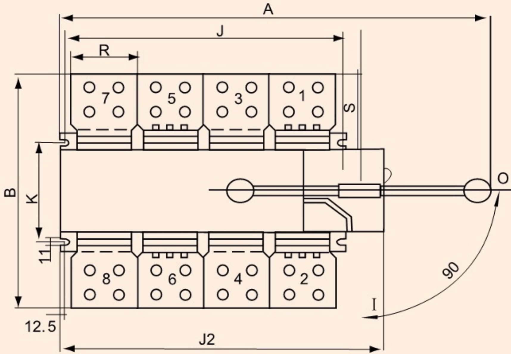
Direct operation on front face 315A/J board
