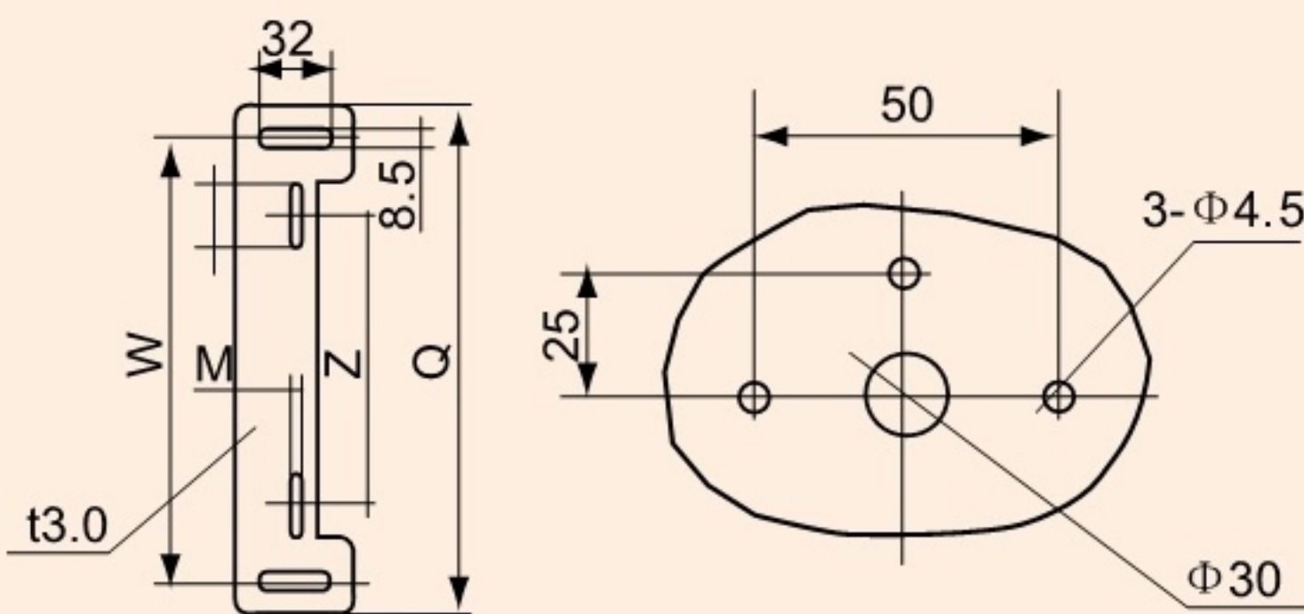
Installation size of handle seat outside board
