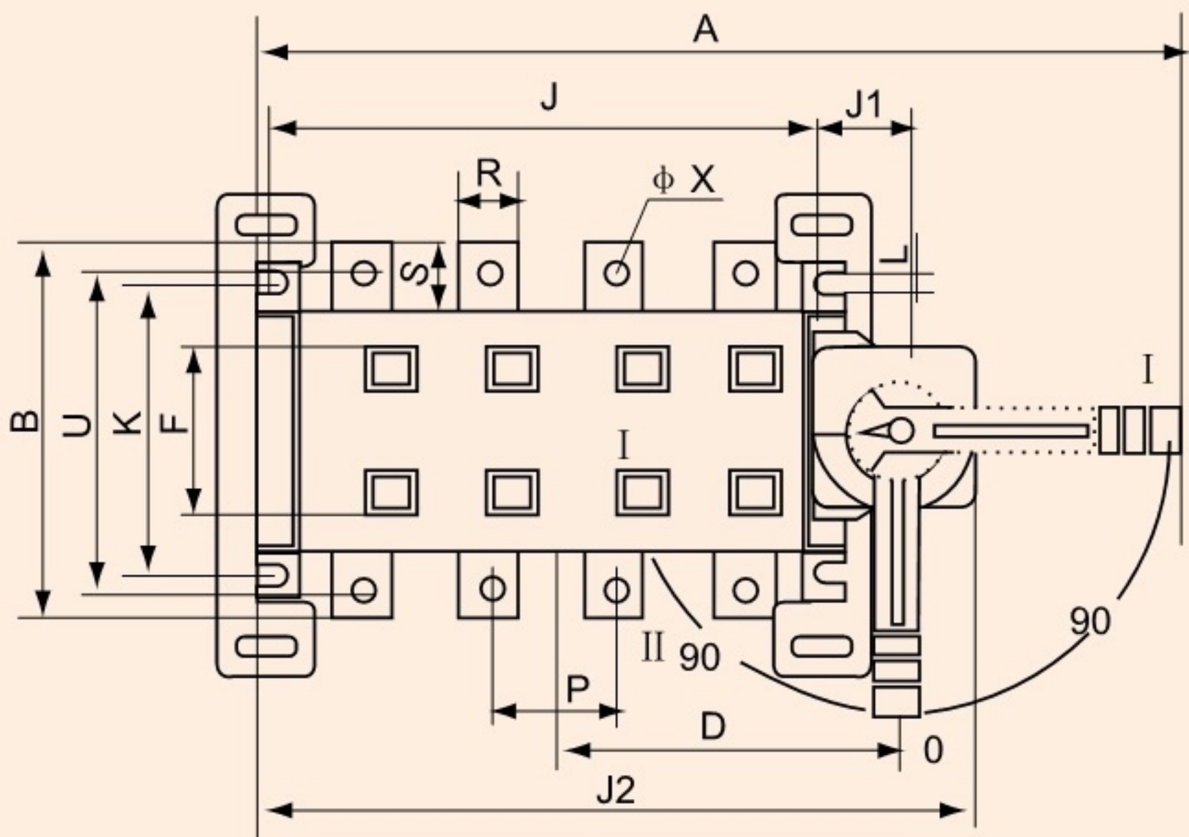
Operation outside 80~630A/J board
